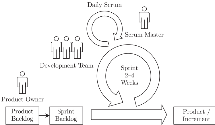
Figure 5. Scrum Process
